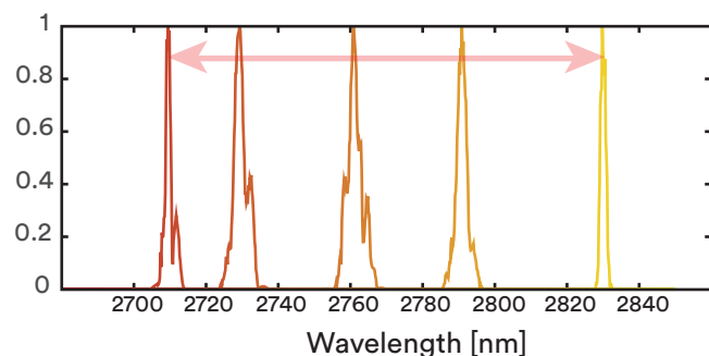
Typical spectrum 3
