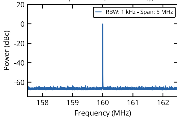
RF spectrum (zoom on f rep )
